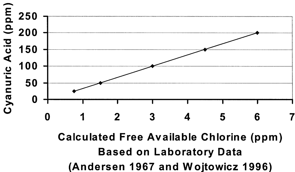
Figure 3 – Minimum Available Chlorine for 30-second 99% Kill Time of S. Faecalis at pH 7.5 and 85°F
