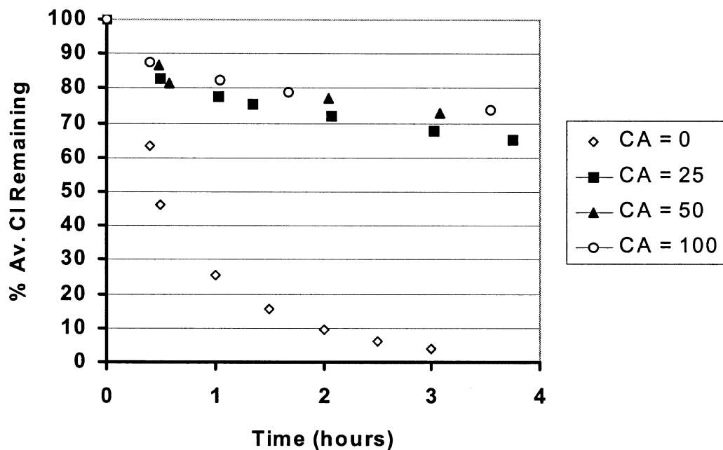
Figure 1 – Effect of Cyanuric Acid on Photochemical Decomposition of Available Chlorine
